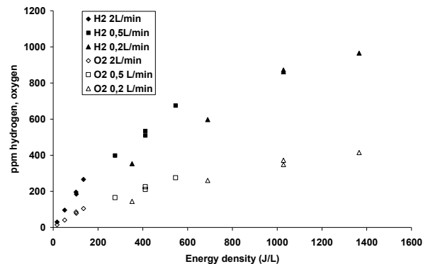
Fig. 1. Hydrogen and oxygen concentration in the effluent gas as a function of energy density and gas flow rate.
