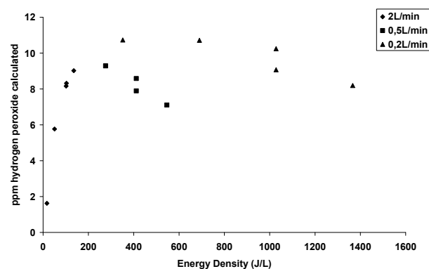
Fig. 2. Hydrogen peroxide production calculated to have been in the effluent gas as a function of energy density and gas flow rate.
