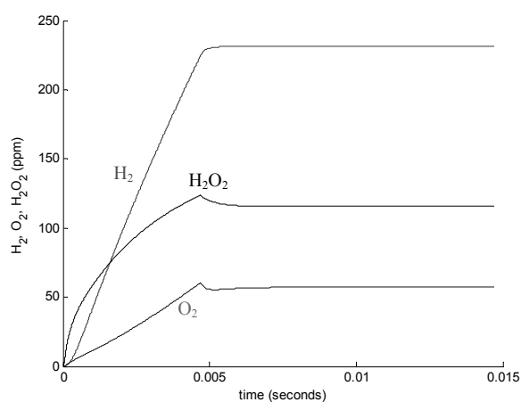
Fig. 4. Result of simulation without dissociation of hydrogen peroxide in the plasma zone.
