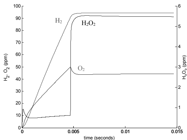
Fig. 5. Result of simulation with dissociation of hydrogen peroxide in the plasma zone for the case of 2L/min and 50J/L.
