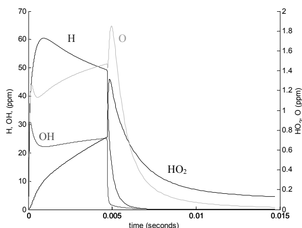
Fig. 6. Radical levels in simulation with the inclusion of dissociation of hydrogen peroxide in the plasma zone.
