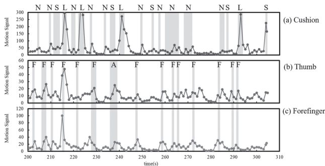
Fig.5 Intensity of motion signals measured by sensors sewn into each location: (a) Cushion, (b) Thumb, (c) Forefinger, and motions confirmed by camera: N, S, L, F and A indicate neck, shoulder, leg, finger and arm motion, respectively.
