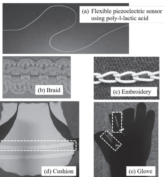
Fig.1 Piezoelectric sensors and fabrics: (a) Flexible piezoelectric sensor using poly-L-lactic acid. (b) Braid of sensor. (c) Embroidery of sensor. (d) Cushion type sensor for detecting heartbeat and body motion. (e) Glove type sensor for detecting thumb and forefinger motions.
